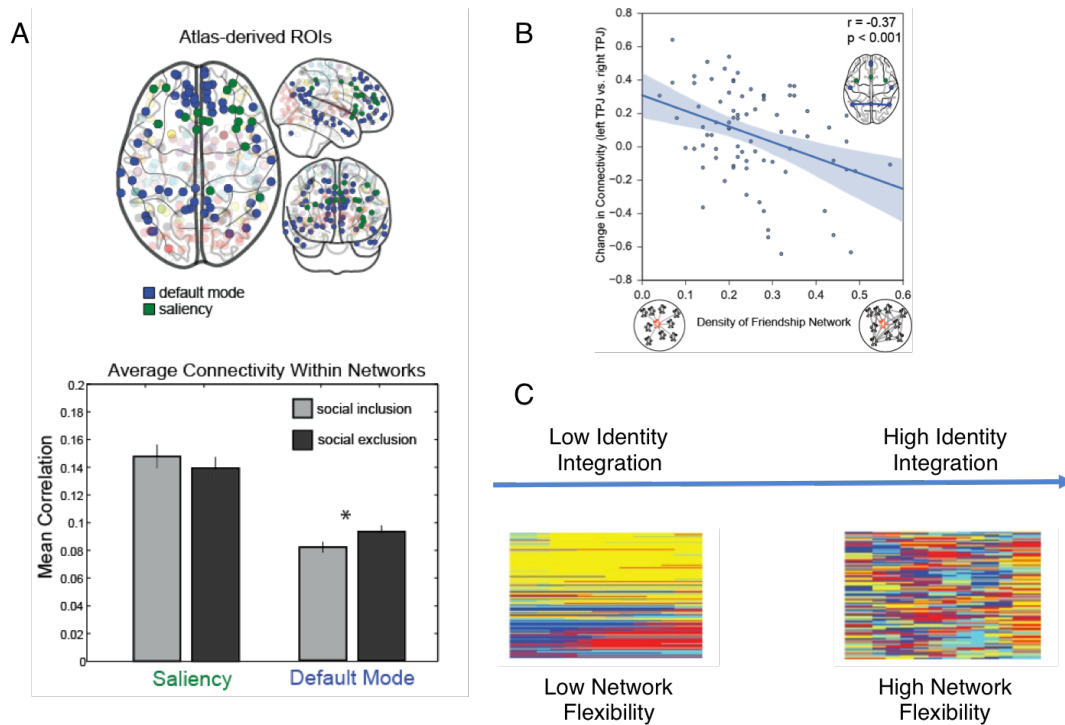
Figure 3. Brain networks and social functioning. Recent work shows that network connectivity within parts of the default mode subnetwork (blue nodes) is greater following social exclusion (3A), and that this effect is moderated by the density of an individual's friendship network (3B; adapted with permission from Schmaelzle et al. (2017)). We suggest that dynamic network methods can advance understanding of social functioning, including how people navigate multiple social identities. People who are better able to integrate multiple social identities may be able to do so, in part, because their brain flexibility adjusts to changing task demands and integrates information between subnetworks. In this case, people high in identity integration would have many brain regions that change communities frequently across time steps (3C).
